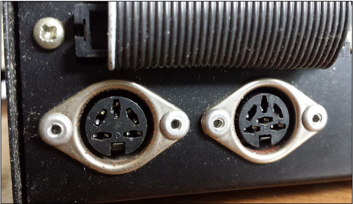
The power connectors on the first MicroPeripherals disk drive – the power supply connects to the 6-pin connector (right) and the second floppy disk drive connects to the five pin (left) connector.
